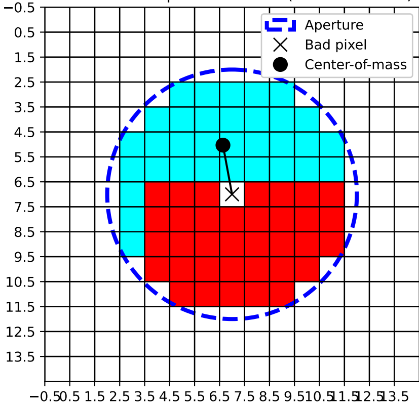
Pixels within aperture radius (masked = red)
