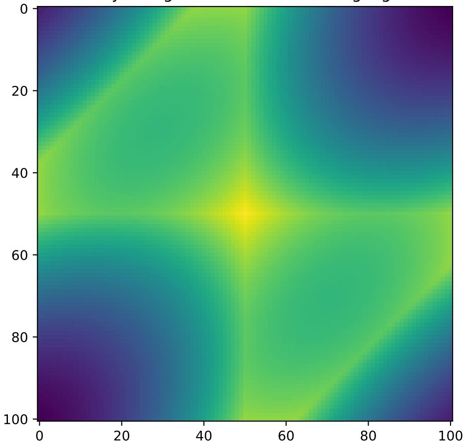
Delaunay triangulation error inside single grid cell
