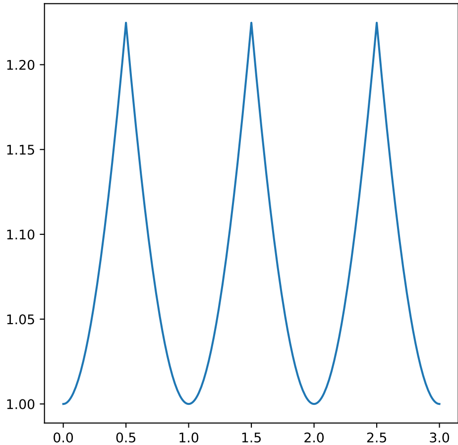
1-D Linear Interpolation Error
