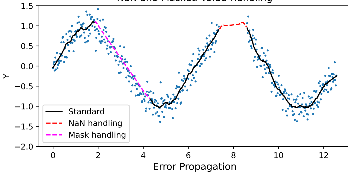
NaN and Masked Value Handling
