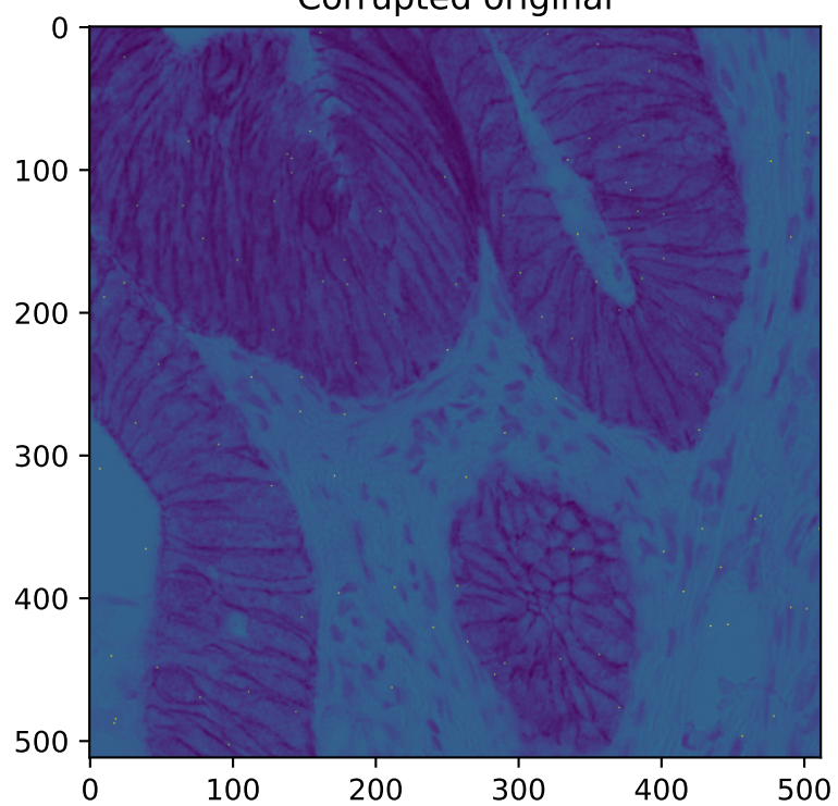
Robust convolution
