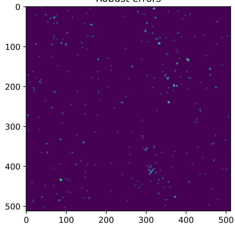
Robust errors
