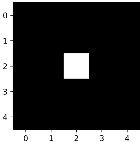
Original Image (5, 5)
