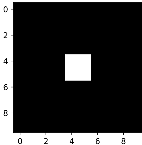
Nearest-Neighbor (10, 10)
