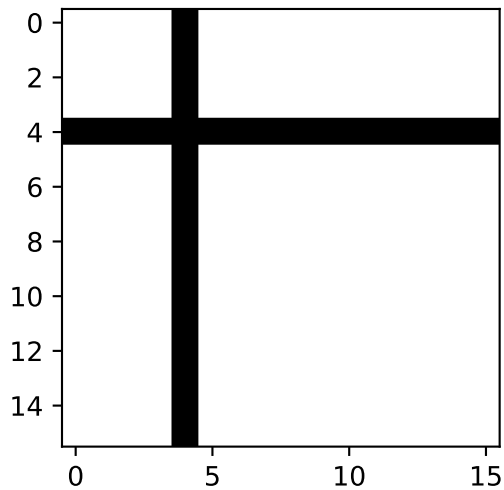
Outliers over full distribution
