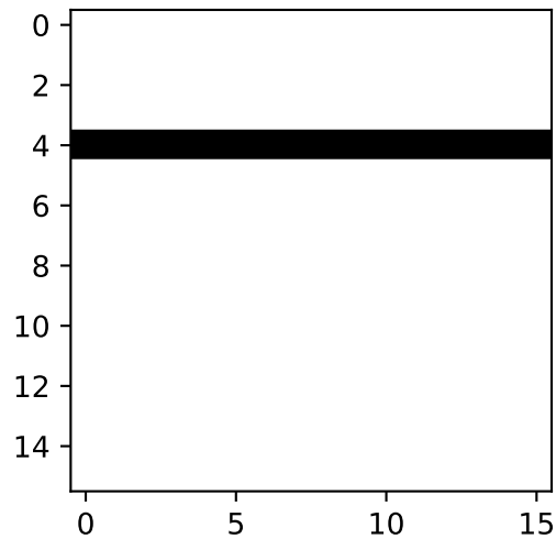
Outliers along dimension 1
