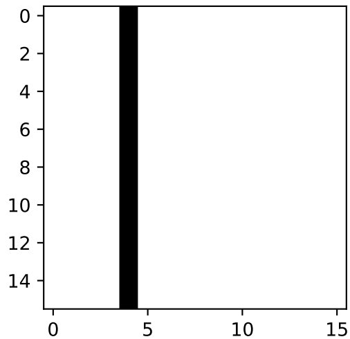
Outliers along dimension 0
