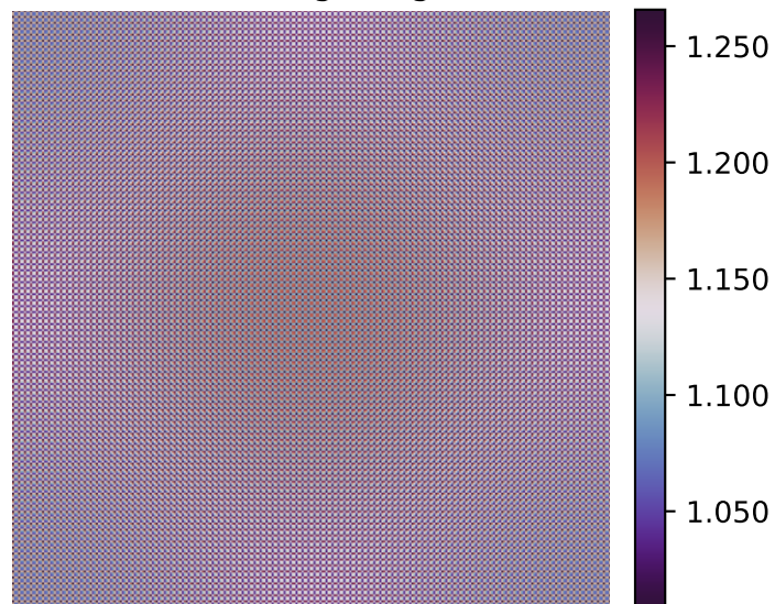
Over-fitting Weights
