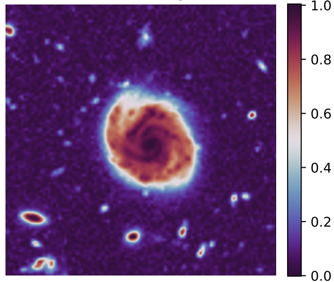
Over-fitting
