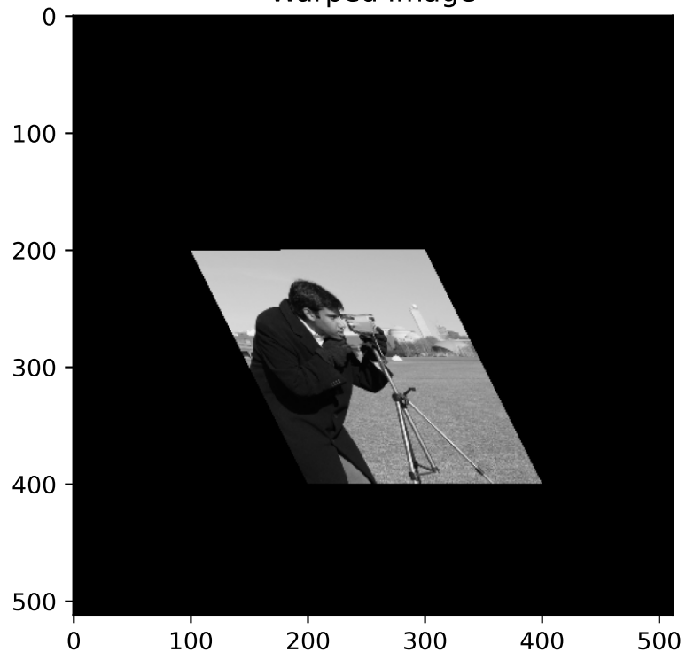
Warped Image
