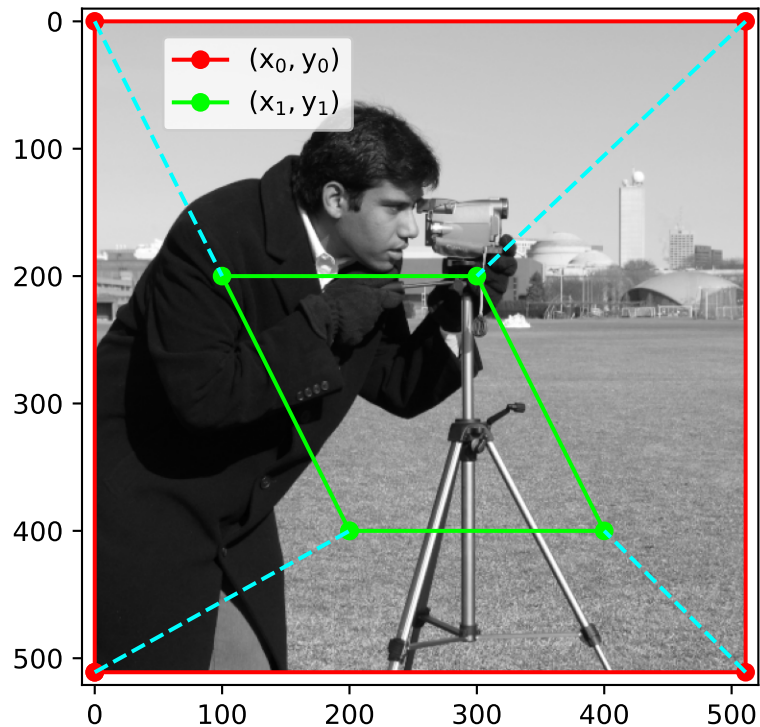
Original Image
