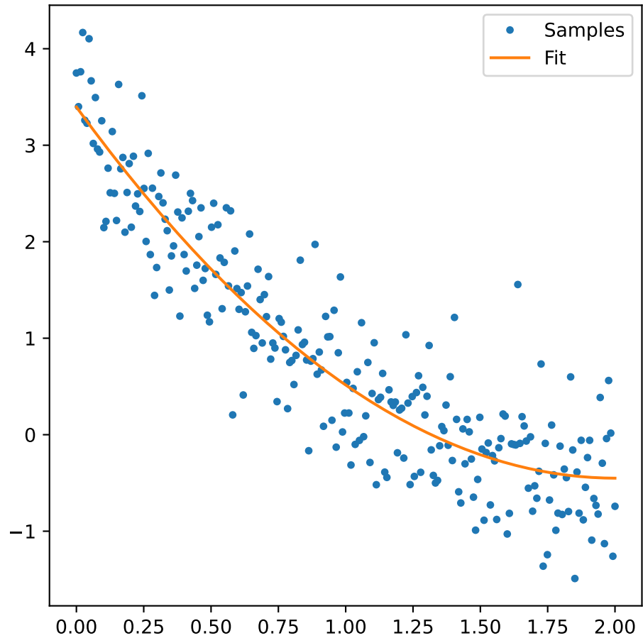
Polynomial fit to noisy data
