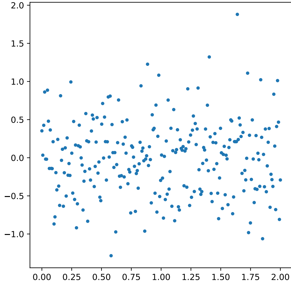
Residuals to the fit
