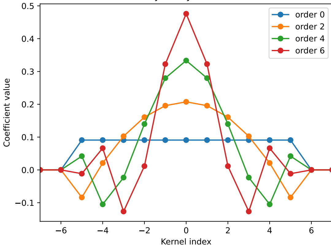
Savitzky-Golay Coefficients
