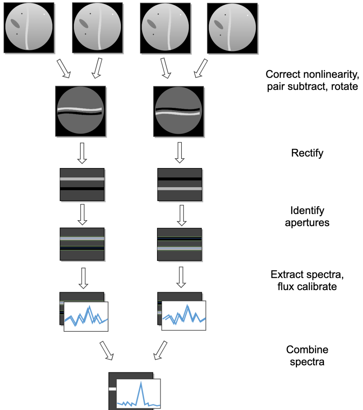
Fig. 4: Processing steps for grism data.
