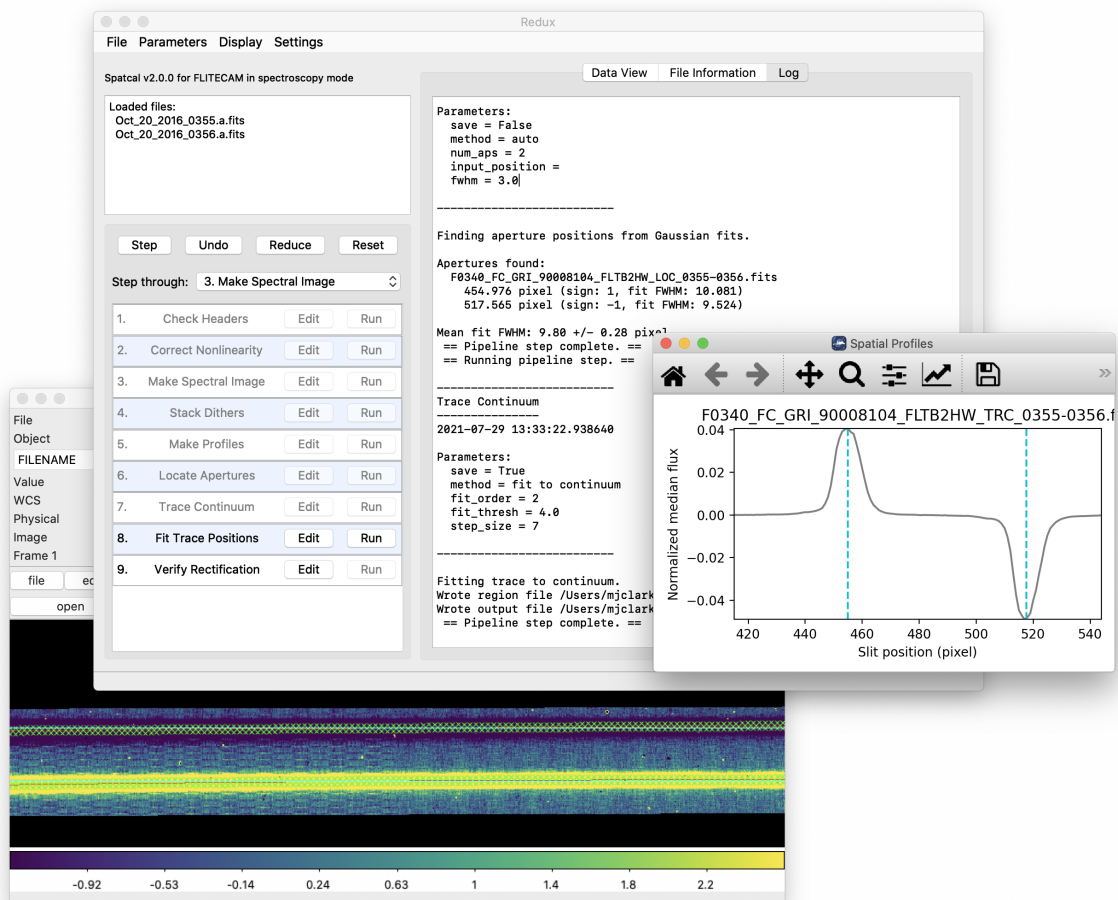
Fig. 22: Spatial mode reduction and diagnostic plots.
