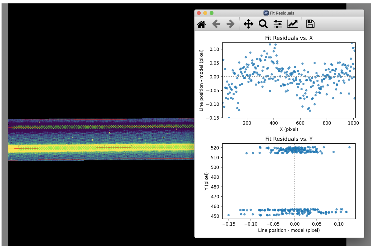
Fig. 24: Spatcal mode fit surface and residuals.
